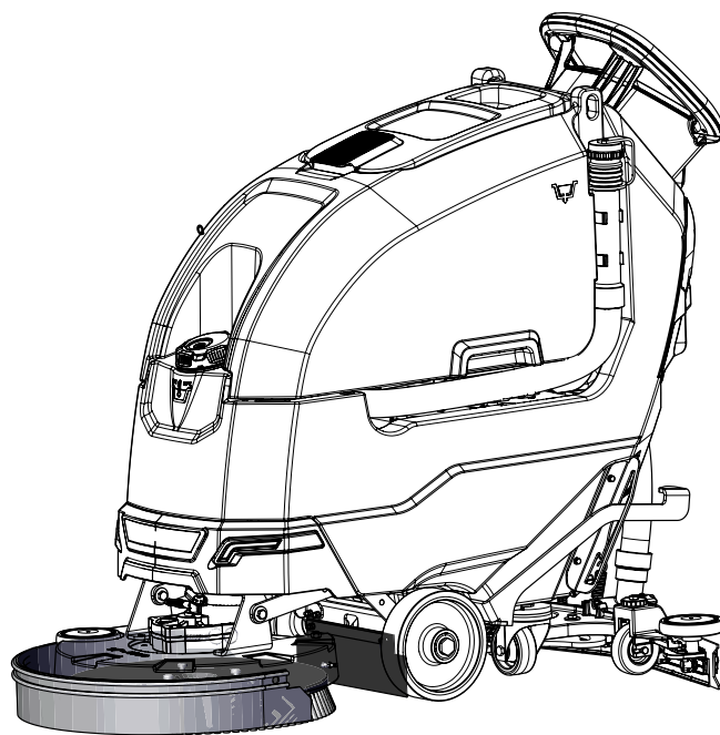
2 - SCRUBBING SYSTEM
