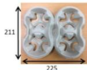
Before Split
