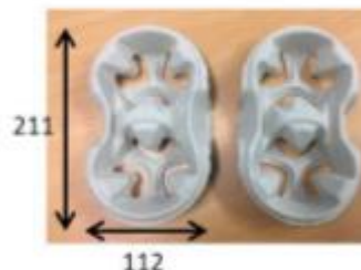
After Split
